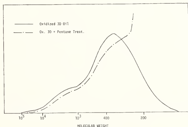
Figure 6. Modified pentane insoluble procedure for the microoxidation test, high coagulant concentration. Microoxidation test conditions: 225 °C, 40 minutes, steel catalyst, 40 \mu\text{l} pentane insoluble procedure: mod. ASTM method, 4 \mu\text{l} of 5 % coagulant in pentane.
